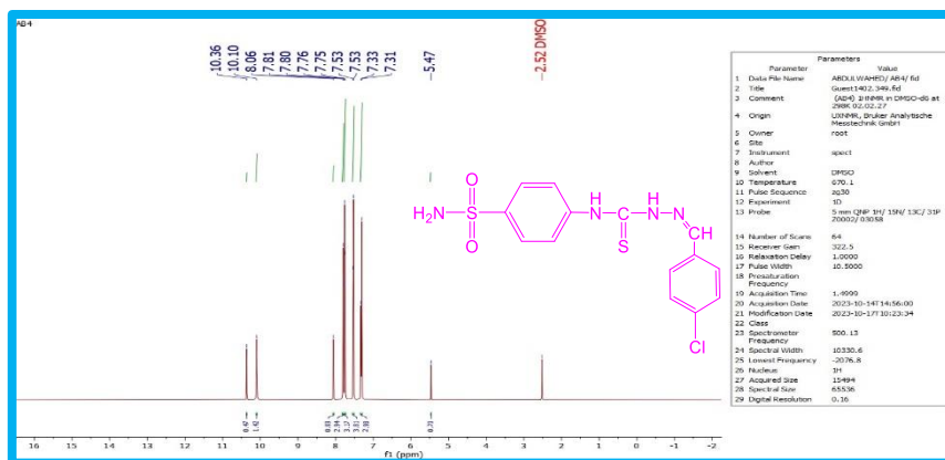
Figure 5. The 1 H-NMR spectrum of the combination (AB4)
