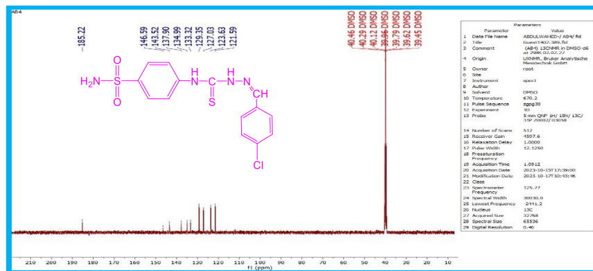
Figure 6. The ^{13}\text{C} -NMR spectrum of the combination (AB4)
